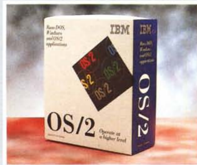
IBM OS/2 2.1
